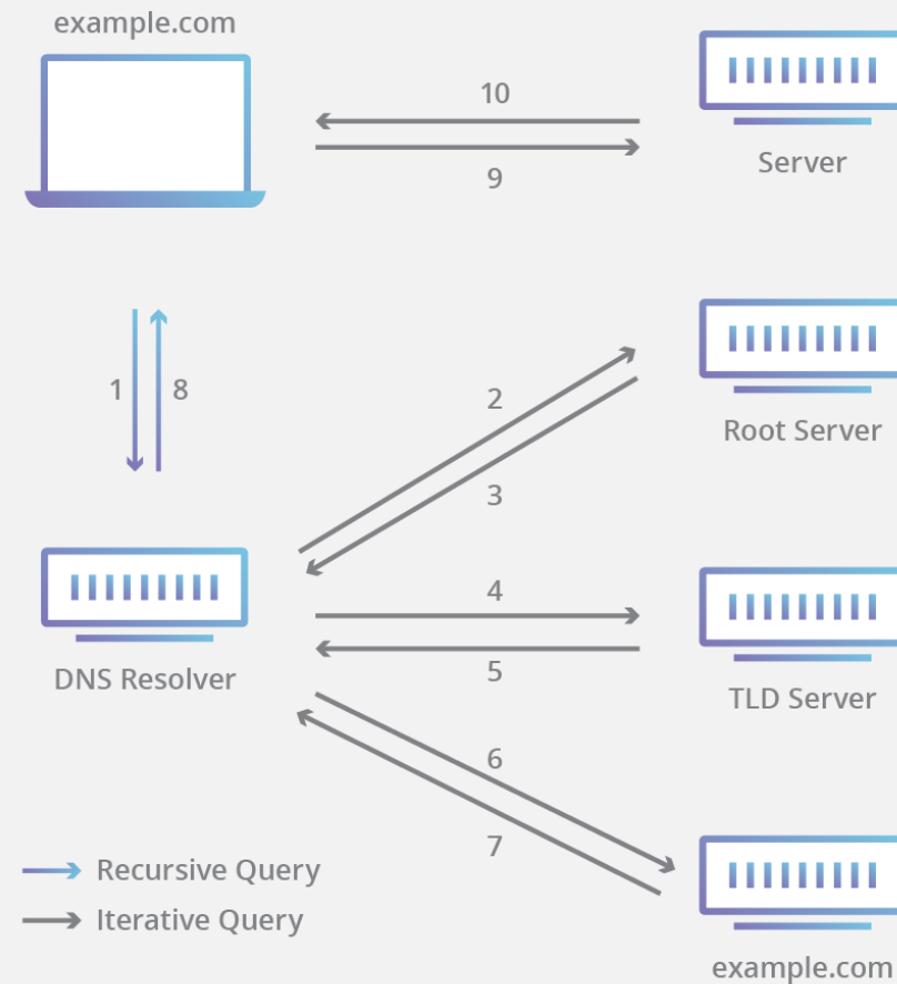
Complete DNS Lookup and Webpage Query
